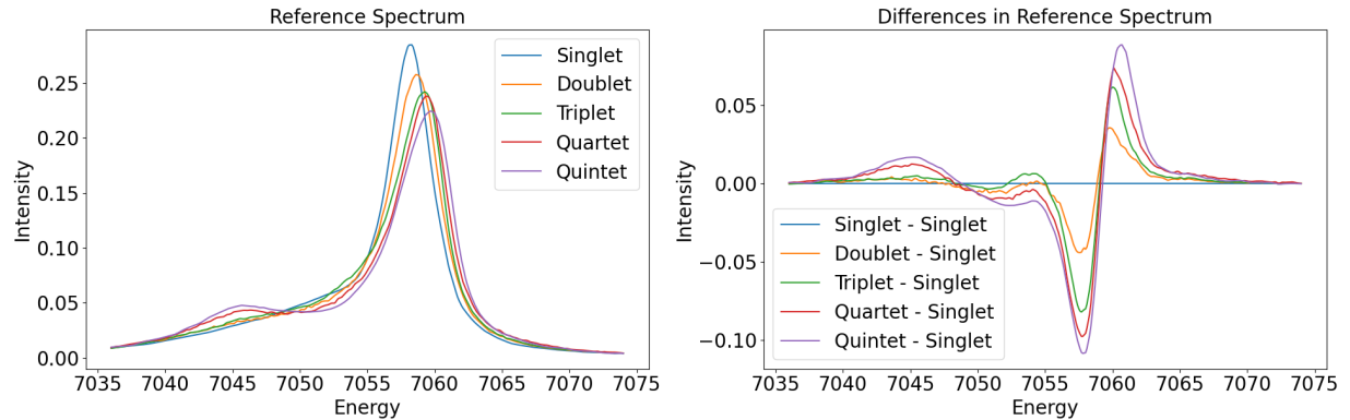
Figure 11: The reference spectra plotted with provided data for different spin states. The reference difference spectra with transient signals plotted with provided data for different transitions.
