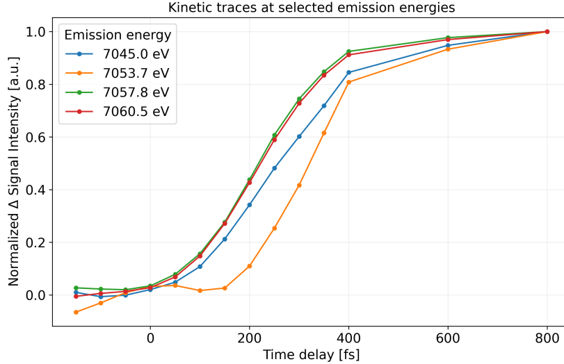
Figure 14: Kinetic traces at selected emission energies.
