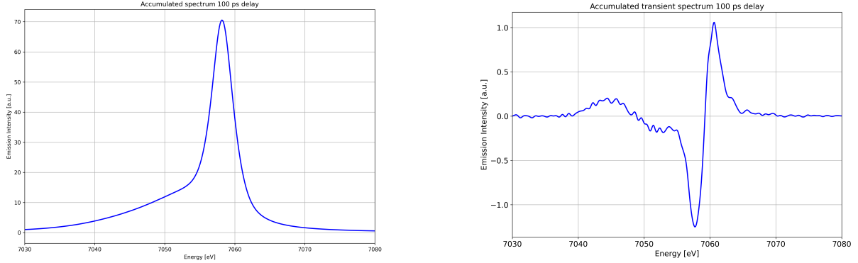
Figure 12: On the left the XES spectrum with the excitation laser on at a delay of 100 ps is plotted. On the right there's the difference spectrum at the same time delay.
