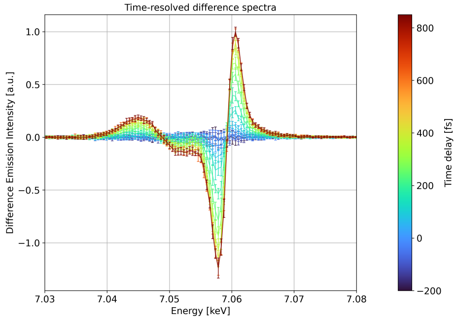
Figure 13: Transient spectra of the X-ray emission at different pump-probe time delays.
