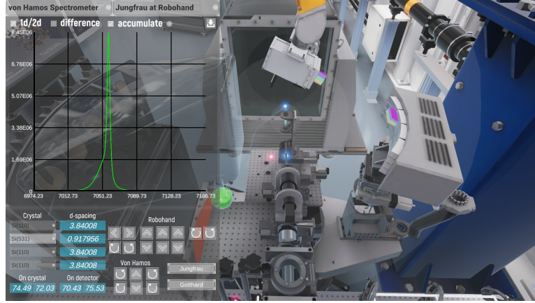
Figure 10: The Vonamos spectrometer in operating position. with the read-out of the Jungfrau detector as well as the settings for the position to the left.
